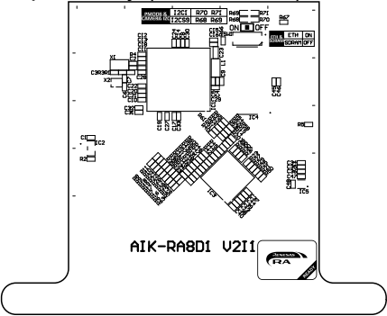
Top Overlay (Scale 1:1.43)
