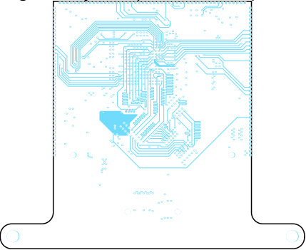
Signal Layer 1 (Scale 1:1.43)
