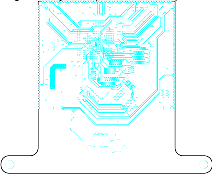
Signal Layer 2 (Scale 1:1.43)
